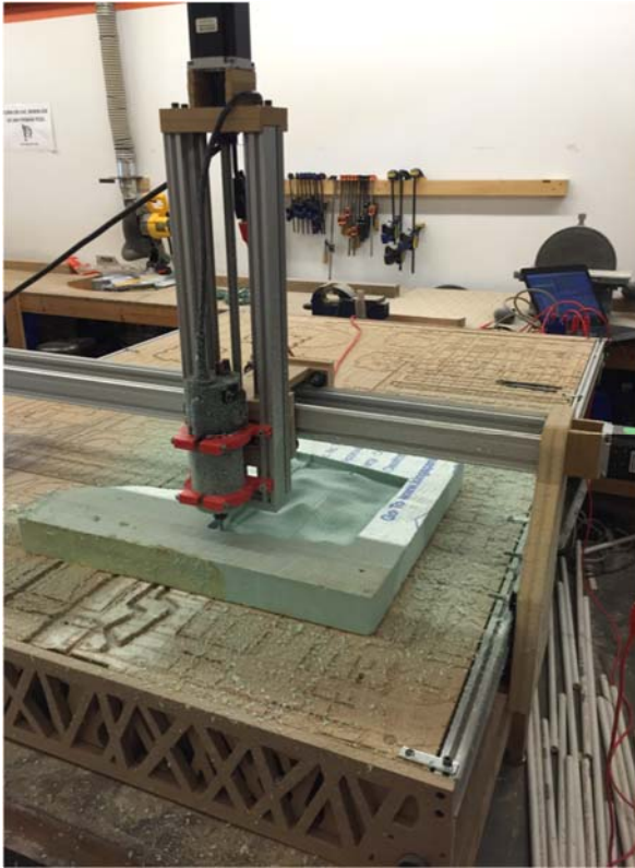
makeLab, CNC built for Polis
